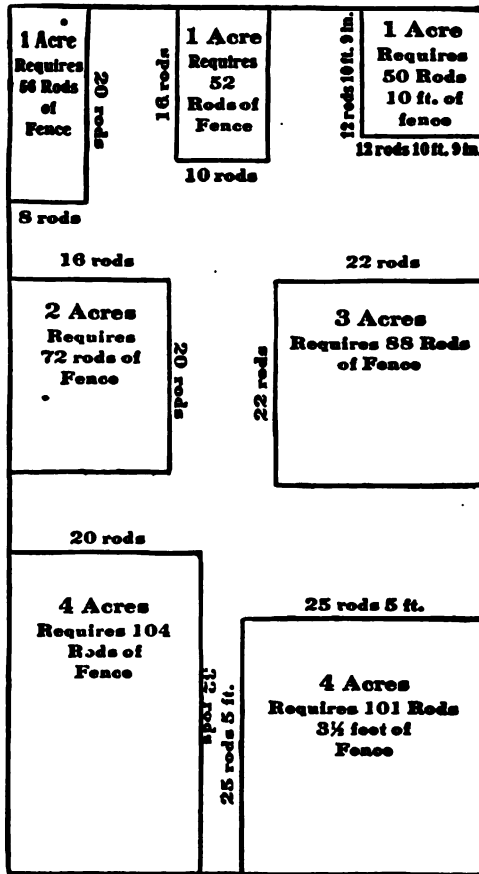
FIG. 17.— Dimensions of 1, 2, 3, and 4 acre lots, and fence required to enclose them. Dimensions given are exact, so that in buying fence, sufficient allowance should be made to cover fence taken up in wrapping around end and corner posts.
